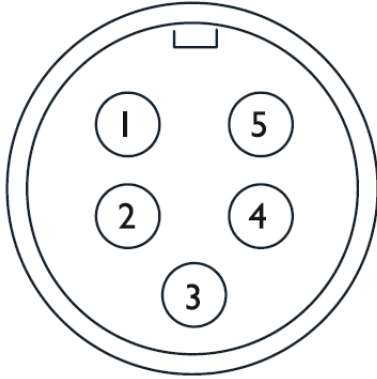
5-Pin Socket
